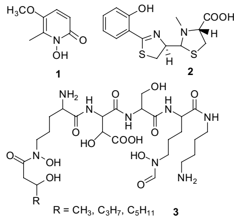
Figure 1. The main siderophores of B. cepacia .
