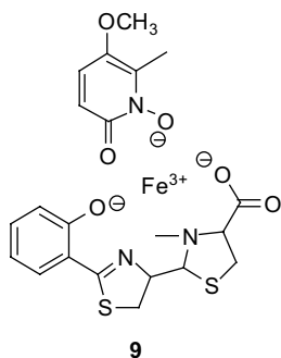
Figure 2. The 1:1:1 complex of iron (III), cepabactin and pyochelin.
