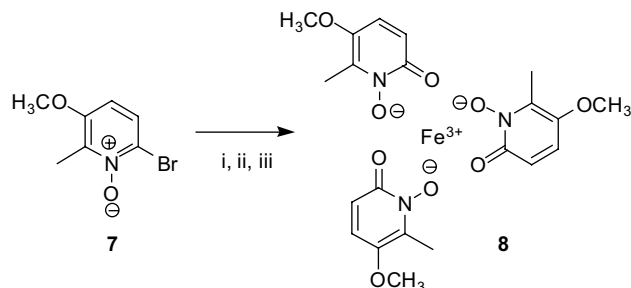
Scheme 2. Reagents and conditions: (i) 10% NaOH aq , \mu -waves; (ii) HCl; (iii) FeCl 3 .
