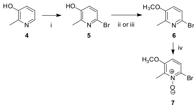
Scheme 1. Reagents and conditions: (i) Br 2 , NaOH aq , 20 °C (yield: 22%); (ii) TMSCHN 2 , MeOH, CH 2 Cl 2 , 20 °C (yield: 91%); (iii) CH 3 I, K 2 CO 3 , acetone, reflux (yield: 95%); (iv) m CPBA, CHCl 3 , reflux (yield: 84%).
